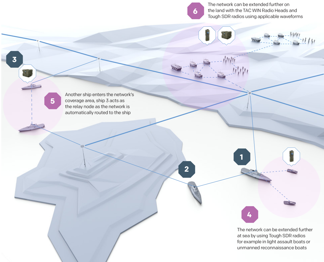
Figure 2: The network can be easily extended both at land and sea, for example with Bittium Tough SDR radios using the same TAC WIN Waveform
